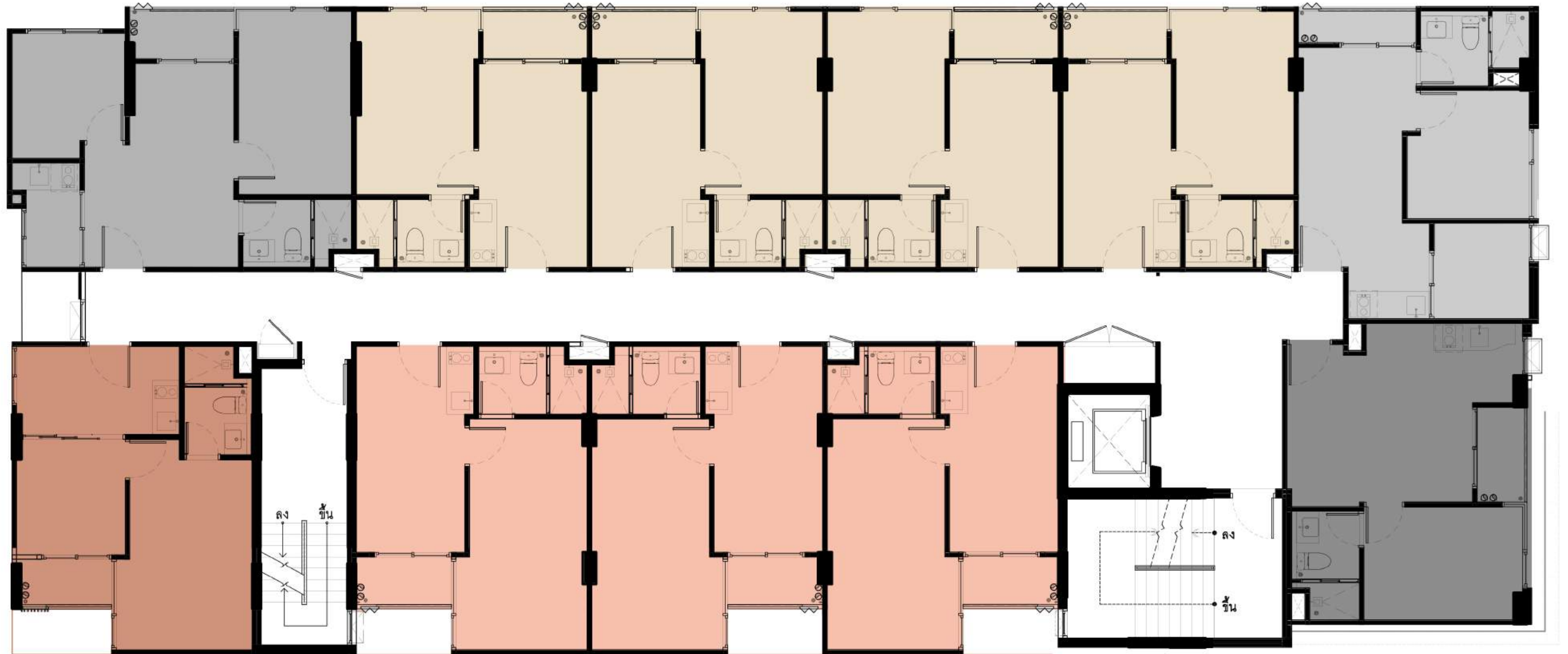
607 TYPE B' 32.50 SQ.M.
